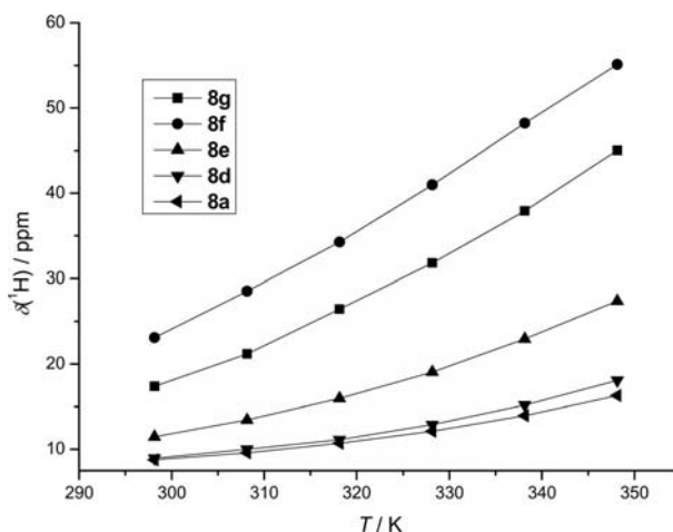
Figure 5. Plot of the chemical shift of protons bound to C23 and C34 versus T for complexes 8a,d-g .
