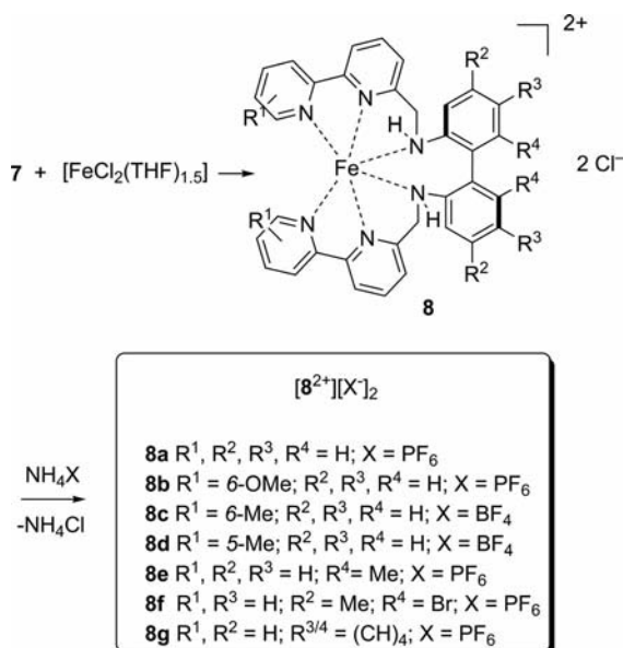
Scheme 3. Synthesis of complexes 8 by treatment of the amines 7 with [\text{FeCl}_2(\text{THF})_{1.5}] .
