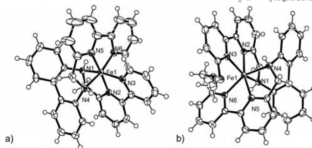
Figure 2. Molecular structures of complexes 8a and 8b in the solid state. Counter ions and solvent molecules are omitted for clarity; probability level is 50%.
