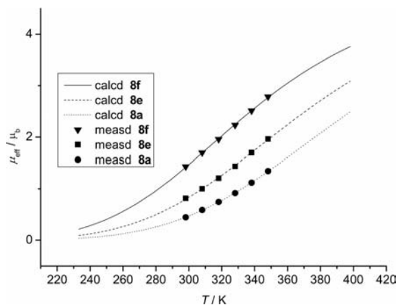
Figure 4. The \mu_{eff} versus T plot of the measured (measd) values in the range 25–75 °C with a 10 K step width and the calculated curves using a regular solution model with best fit parameters given in the text.
