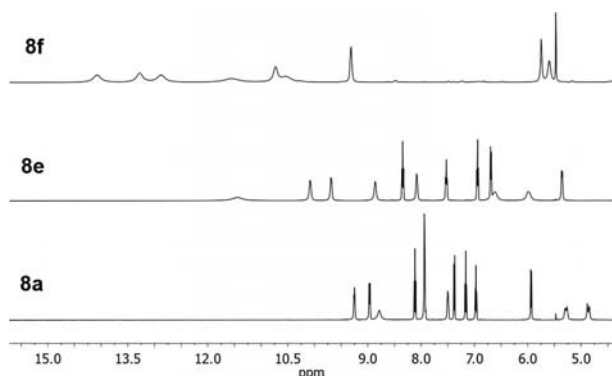
Figure 3. Downfield region of ^1H NMR spectra of complexes 8a , 8e and 8f at 25° in CD_3CN solution.
