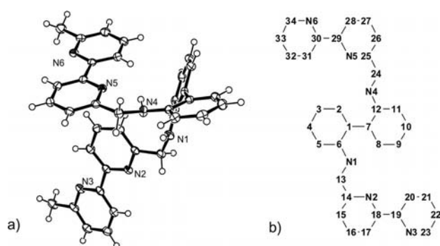
Figure 1. ORTEP diagram of the molecular structure of 7c in the solid state and the applied numbering scheme for amines 7 and complexes 8 .
