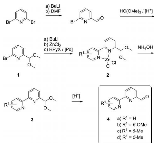
Scheme 1. Synthesis of 4a–d by a Negishi cross-coupling reaction (DMF = dimethylformamide).
