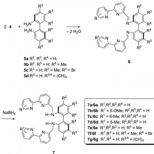
Scheme 2. Synthesis of the hexadentate molecules 7 with \text{AB}_2 structure by condensation of 2,2'-diaminobiphenyls ( 5 ) with 2,2'-bipyridine-6-carbaldehydes ( 4 ) and subsequent reduction with \text{NaBH}_4 .
